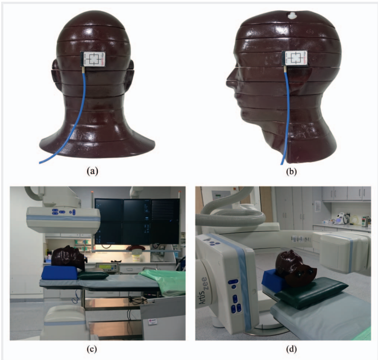
► Fig. 1 Setup for measuring the conversion factors on the head phantom. Placement of the silicon semiconductor detector at a the undertable or p.-a. projection and b the overtable or lateral projection. Position of the head phantom relative to the C-arm at c the undertable or p. a. projection and d the overtable or lateral projection.
