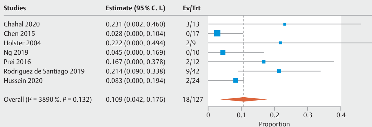
► Fig. 3 Pooled analysis of 7-day rebleeding rate after use of hemostatic powders. Rate of bleeding recurrence within 7 days from the index procedure was 10.9% (95%CI 4.2%–17.6%), with evidence of moderate heterogeneity ( I^2 = 38.9\% ). CI, confidence interval.
