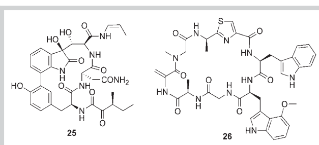
Fig. 7 Structures of cyclic peptides as proteasome inhibitors.
