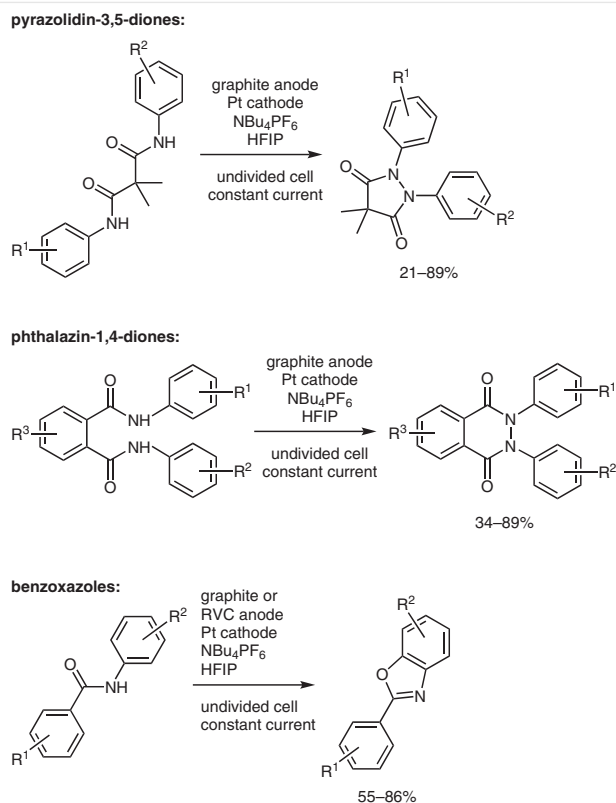
Scheme 11 Anodic synthesis of pyrazolidin-3,5-diones and phthalazin-1,4-diones and benzoxazoles through intramolecular coupling in HFIP. 46–49
