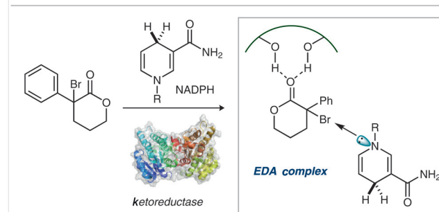
Scheme 3 Mechanistic studies
