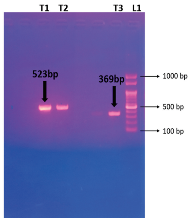
Fig. 1 Image of gel electrophoresis of PCR for detecting aminoglycoside modifying enzyme (AME) gene. Band at 523bp (T1&T2) represents the presence of aph(3')-IIIa gene and band at 369bp (T3) represents presence of aac(6')-Ie-aph(2'')-Ia gene. L1 is the 100bp ladder. PCR, polymerase chain reaction.
