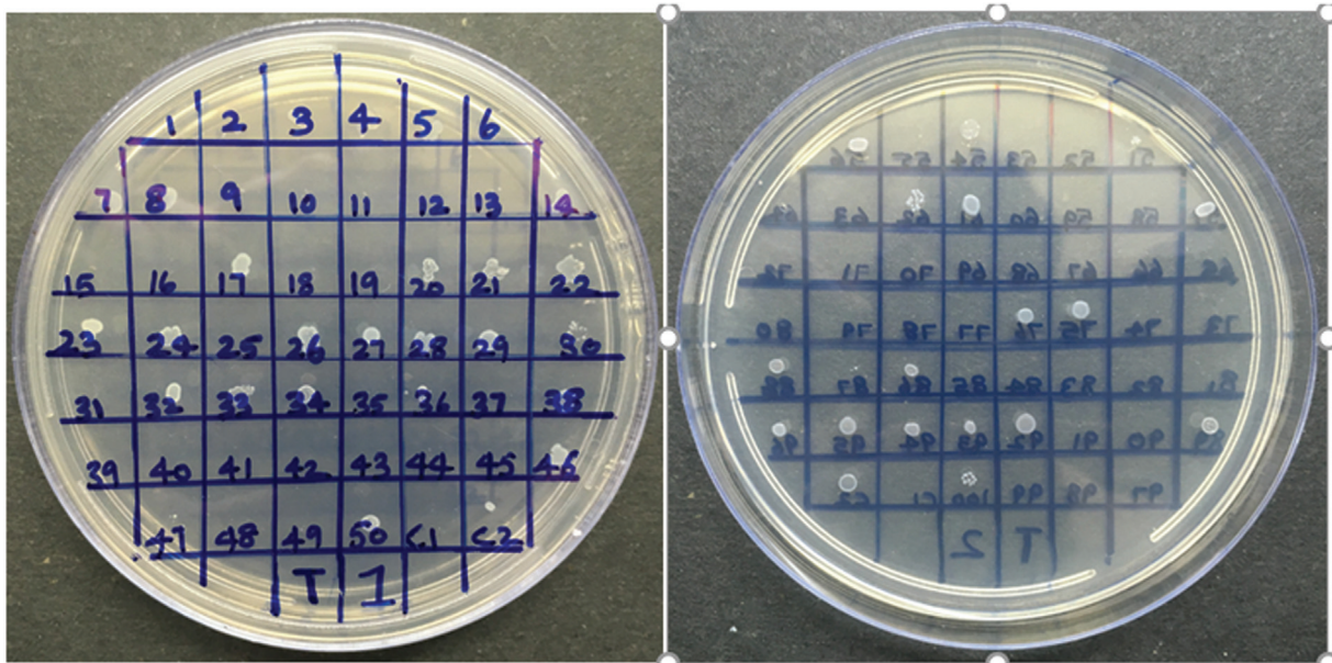
Fig. 2 Image of minimum inhibitory concentration (MIC) testing for high level gentamicin (> 500 µg/mL); done by the agar dilution method.
