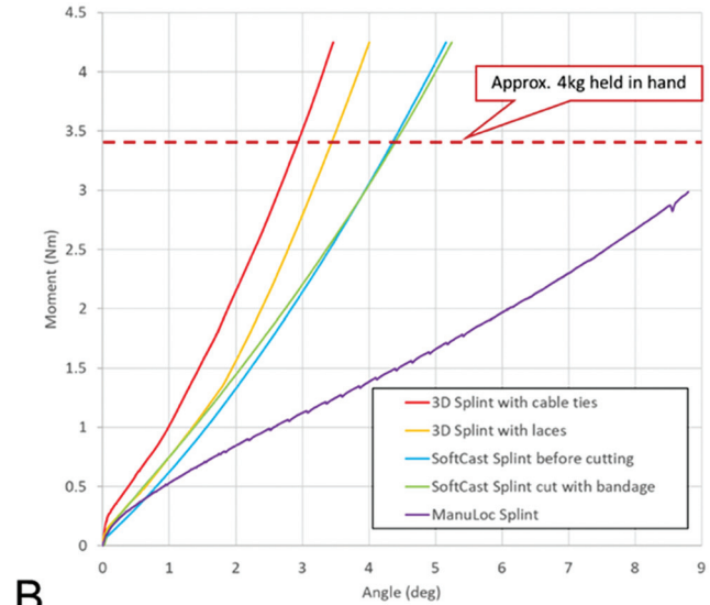
Fig. 2 (A) Test bench used to measure the brace stiffness in flexion and extension (forced wrist extension illustrated). (B) Stiffness curves for forced extension, representing the bending moment as function of the angular rotation: 3D splint with cable ties (red), lace (yellow), circular SoftCAST, split SoftCAST with bandage, and prefabricated ManuLoc splint. Reference bending moment for stiffness value determination (dashed red horizontal line).
