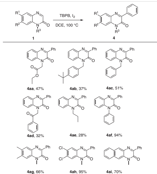
Scheme 7 Substrate scope of quinoxalin-2(1 H )-ones. Reagents and conditions: 1a (0.3 mmol), I 2 (0.02 equiv.), TBPB (5.0 equiv.), solvent (2.0 mL), sealed tube. 27
