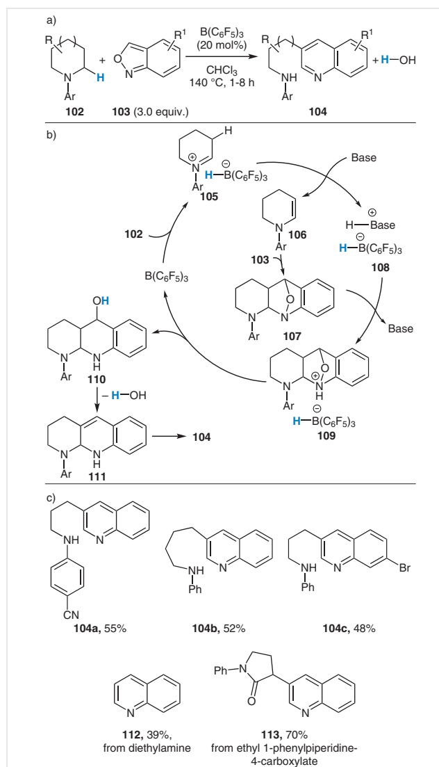
Scheme 13 Borane-mediated hydride abstraction for the conversion of benzo[ c ]isoxazoles into functionalized quinolines
