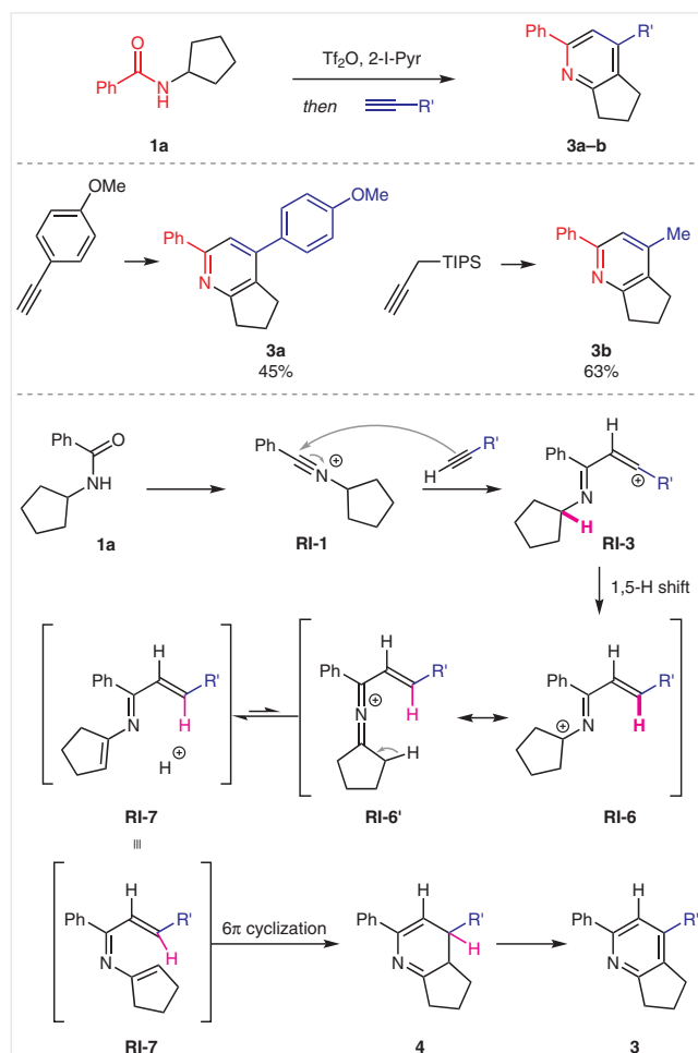
Scheme 5 Unexpected formation of a pyridine core
