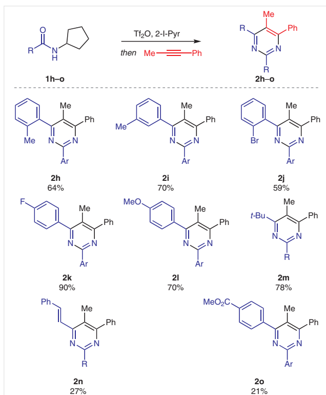
Scheme 4 Scope of the amide. Reagents and conditions: amide (0.6 mmol, 3 equiv), 2-iodopyridine (3 equiv), 1,2-dichloroethane (3 mL), 0 °C; addition of \text{TiF}_4 (3 equiv), after 15 min, addition of alkyne (1 equiv); 90 °C, 18 h. Quench: saturated \text{NaHCO}_3 solution, stirring, 1 h, r.t.
