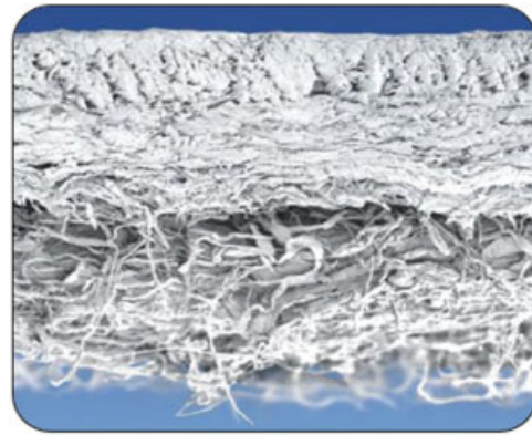
Fig. 1 Bilayer structure.
