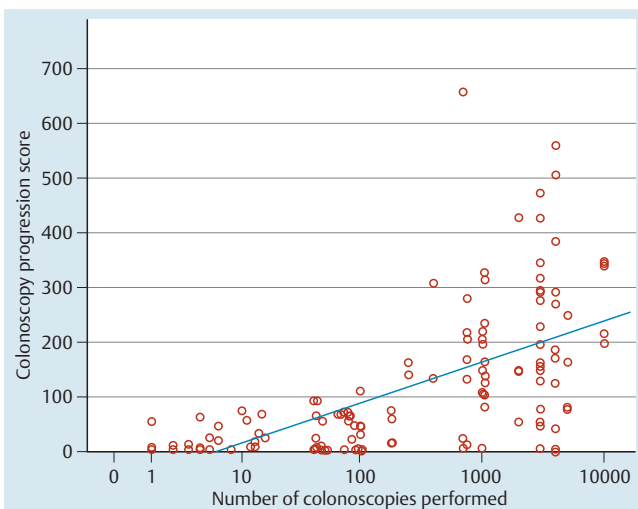
Fig. 3 Performance score according to the level of experience as number of prior procedures. Each dot represents a score correlated to experience.
