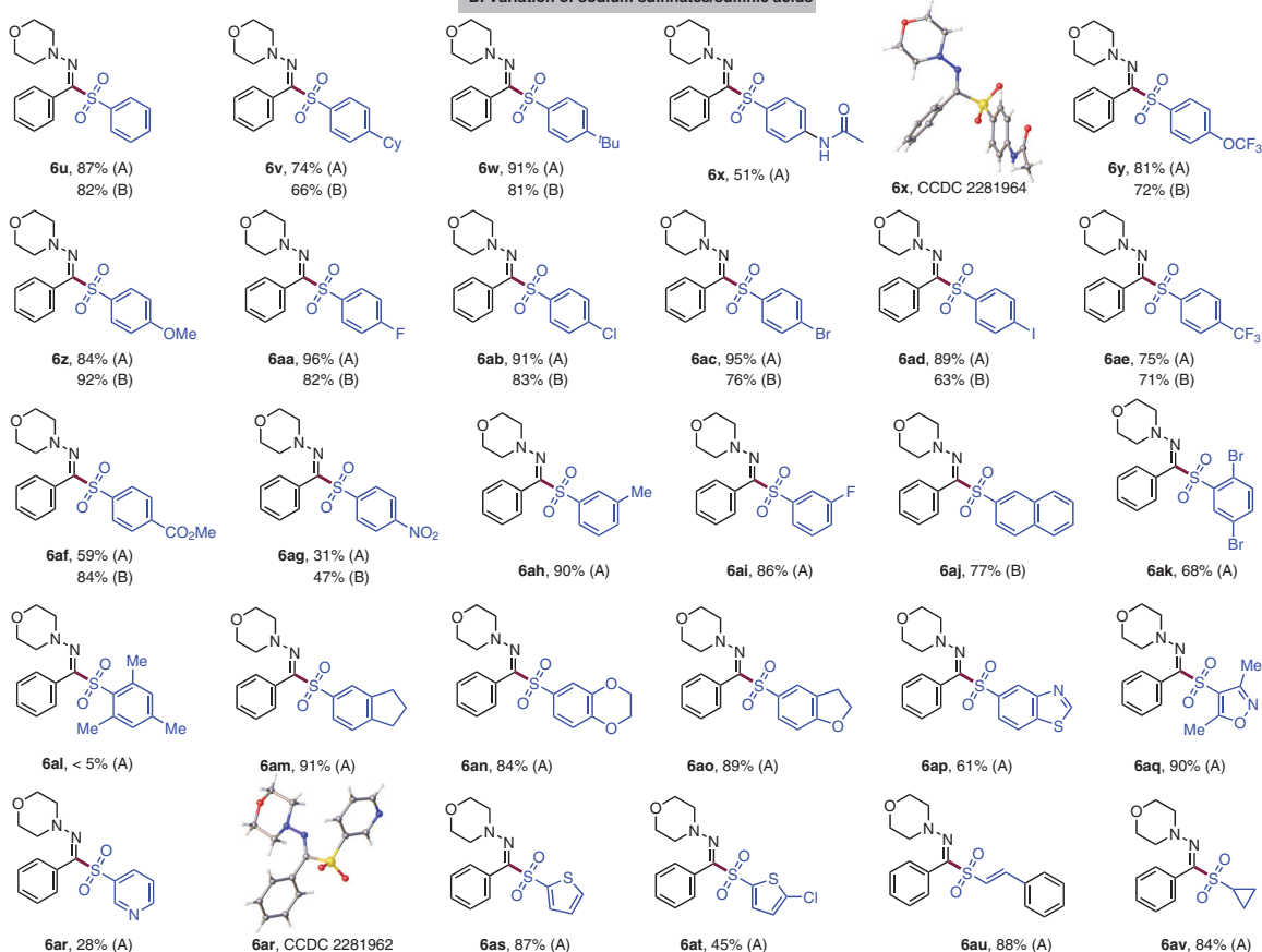
Scheme 4 Substrate scope. Conditions A: Graphite Felt anode (10 × 15 × 2 mm 3 ), Pt cathode (10 × 10 × 0.2 mm 3 ), 1 (0.2 mmol), 2 (0.4 mmol), n Bu 4 NBF 4 (0.05 M), MeCN/H 2 O (1:1 v/v, 6 mL), room temperature (ca. 27 °C), 10 mA. Conditions B: Graphite Felt anode (10 × 15 × 2 mm 3 ), Pt cathode (10 × 10 × 0.2 mm 3 ), 1 (0.2 mmol), 3 (0.3 mmol), n Bu 4 NBF 4 (0.05 M), MeCN/H 2 O (1:2 v/v, 6 mL), room temperature (ca. 27 °C), 10 mA. Isolated yields given.
