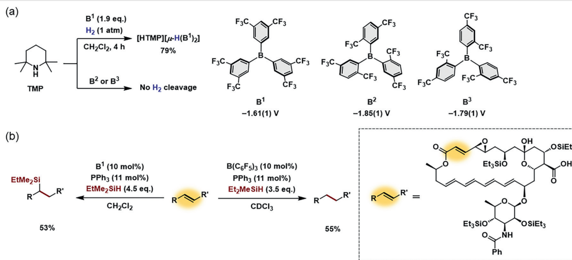
Scheme 1 (a) Heterolytic cleavage of \text{H}_2 via the combination of TMP and \text{B}^1 – \text{B}^3 , with their formal reduction potentials (vs. [\text{FeCp}_2]^{0/+} [V]) and (b) the reduction of a bioactive compound using \text{B}^1 or \text{B}(\text{C}_6\text{F}_5)_3 .
