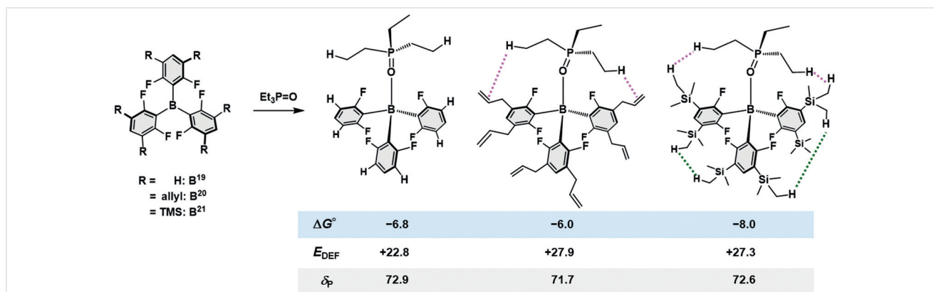
Scheme 4 Comparison of theoretical parameters for the formation of Et 3 P=O- B n ( n = 19–21) adducts, i.e. relative Gibbs energies ( \Delta G^\circ in kcal mol -1 with respect to [ B n + Et 3 P=O]), and deformation energies ( E_{\text{DEF}} in kcal mol -1 ). The chemical shifts in 31 P NMR, \delta_{\text{P}} , obtained in the reaction between B 19 – B 21 and Et 3 P=O (0.3 eq.) in CH 2 Cl 2 are also given.
