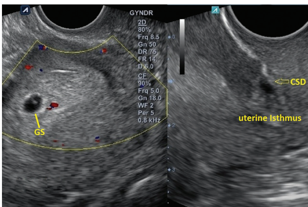
Fig. 4 TVUS reveals a 5-week intrauterine gestational sac with an isthmocele (arrow). The RMT/AMT ratio was <50\% . In such cases, the risk of PAS increases if the future placenta is anterior and low lying. The niche can retain POC in the event of spontaneous abortion or if MTP is chosen. AMT, adjacent myometrial thickness; CSD, cesarean scar defect; GS, gestational sac; MTP, medical termination of pregnancy; PAS, placenta accreta spectrum; POC, products of conception; RMT, residual myometrial thickness; TVUS, transvaginal ultrasound.
