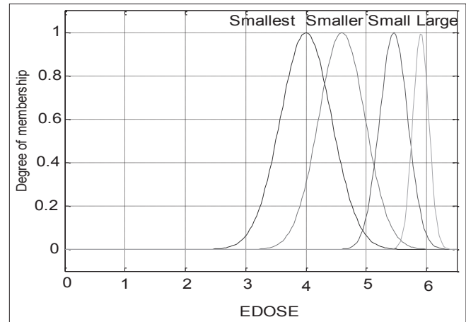
Figure 4: The membership function for the output effective dose (EDOSE)
