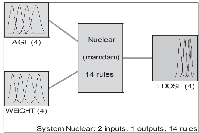
Figure 2: The block diagram of the fuzzy inference system
