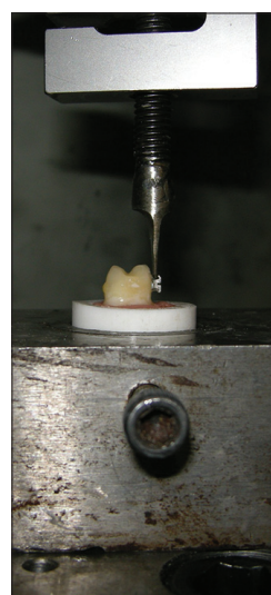
Figure 1: Position of the tooth and bracket in the Zwick testing machine, prior to the debonding process
