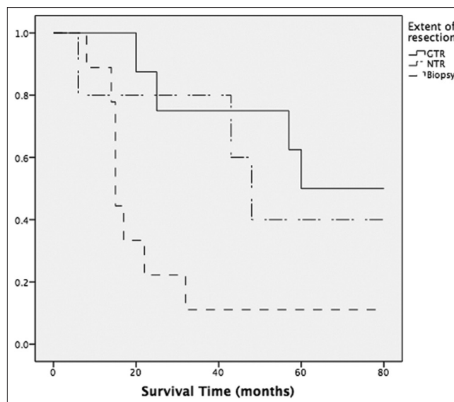
Figure 2: Kaplan-Meier plot for extent of resection
