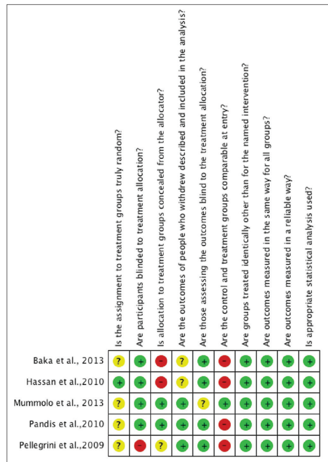
Figure 3: Summary of the risk of bias scored according to Meta-analysis of Statistics Assessment and Review Instrument checklist as (+) YES; (-) NO; (?) unclear
