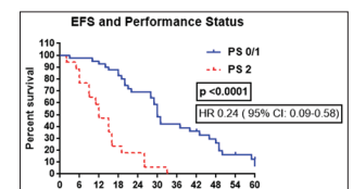
Figure 2: Kaplan–Meier estimates showing effect of performance status on event-free survival
