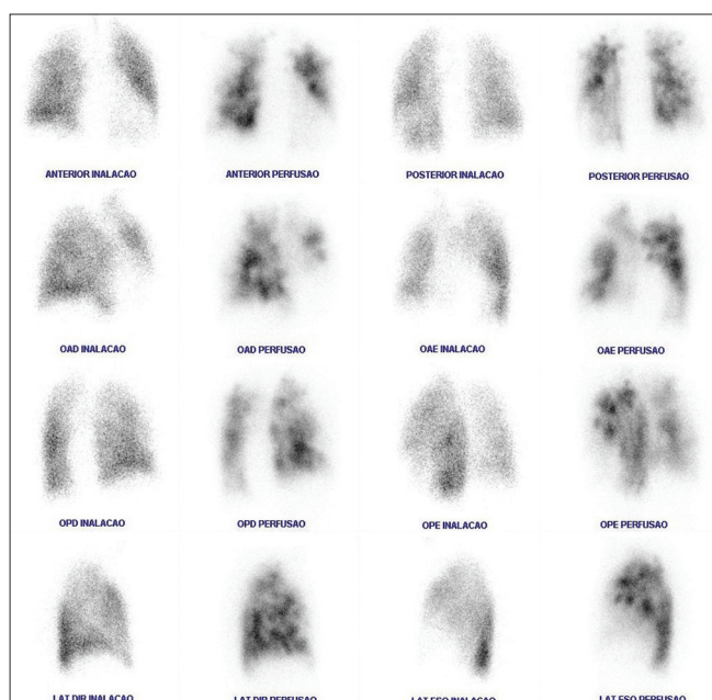
Figure 1: Ventilation-perfusion scintigraphy
